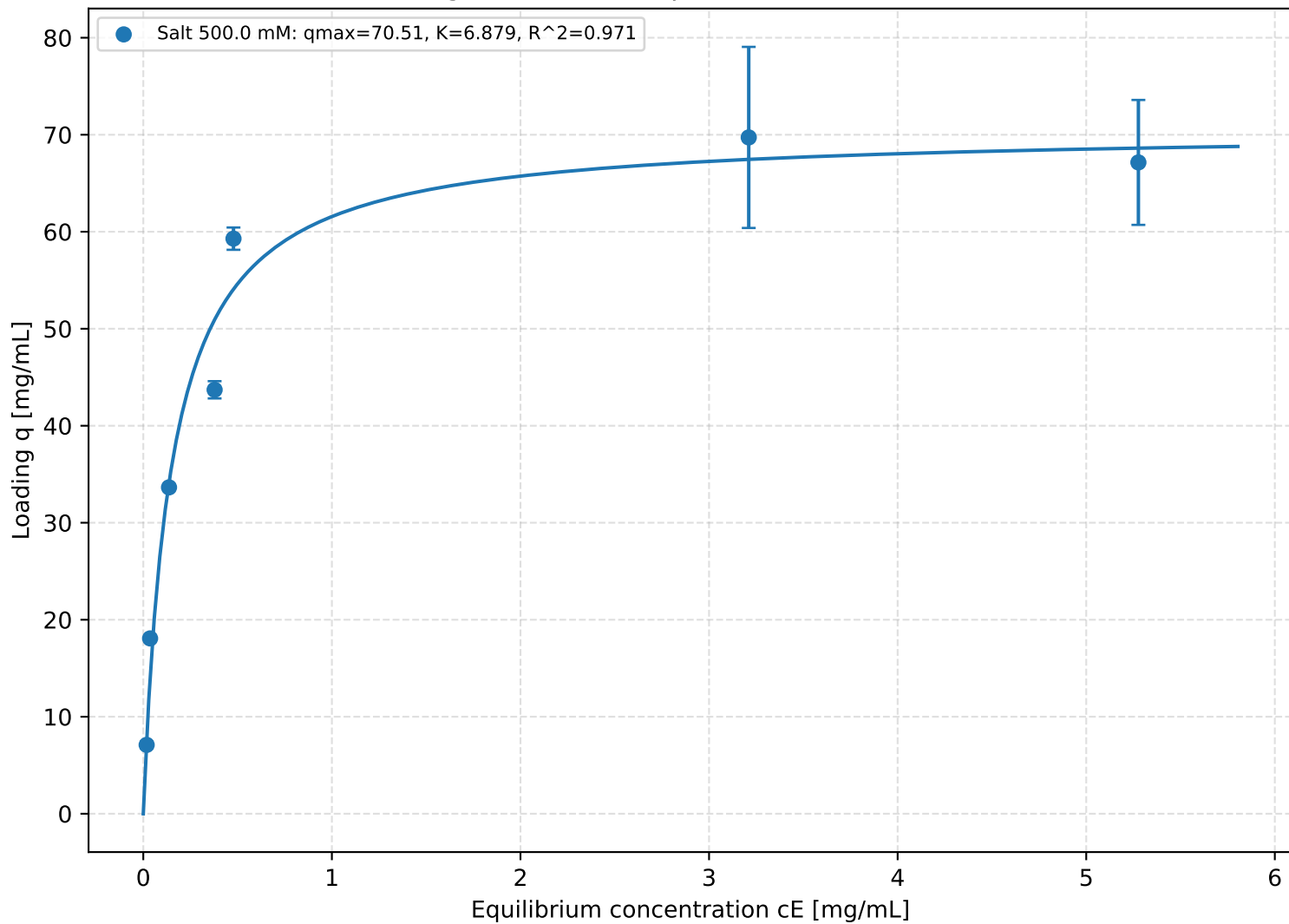
Loading Isotherms - Experiment 5024 at 280 nm
